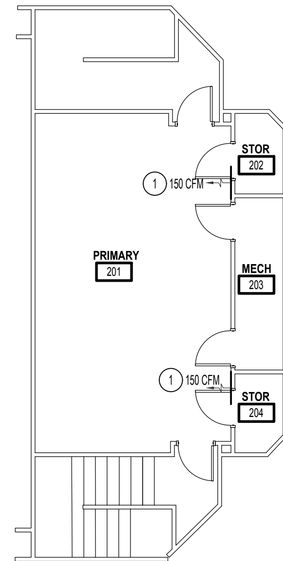
MECHANICAL PLAN SCALE: 1/8" = 1'-0"
